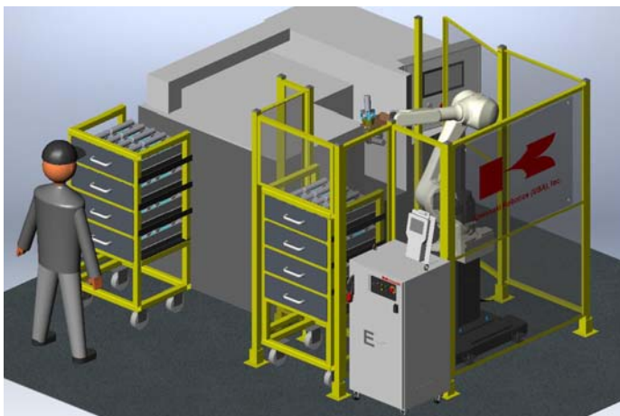
Vertical Drawer Roller Cart System
