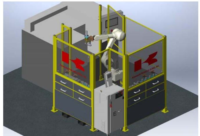
Dual Stationary Drawer System
